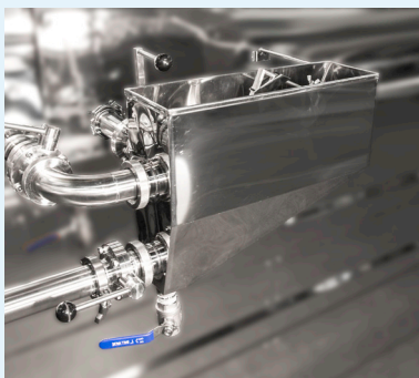
Transfer box with sediment trap
